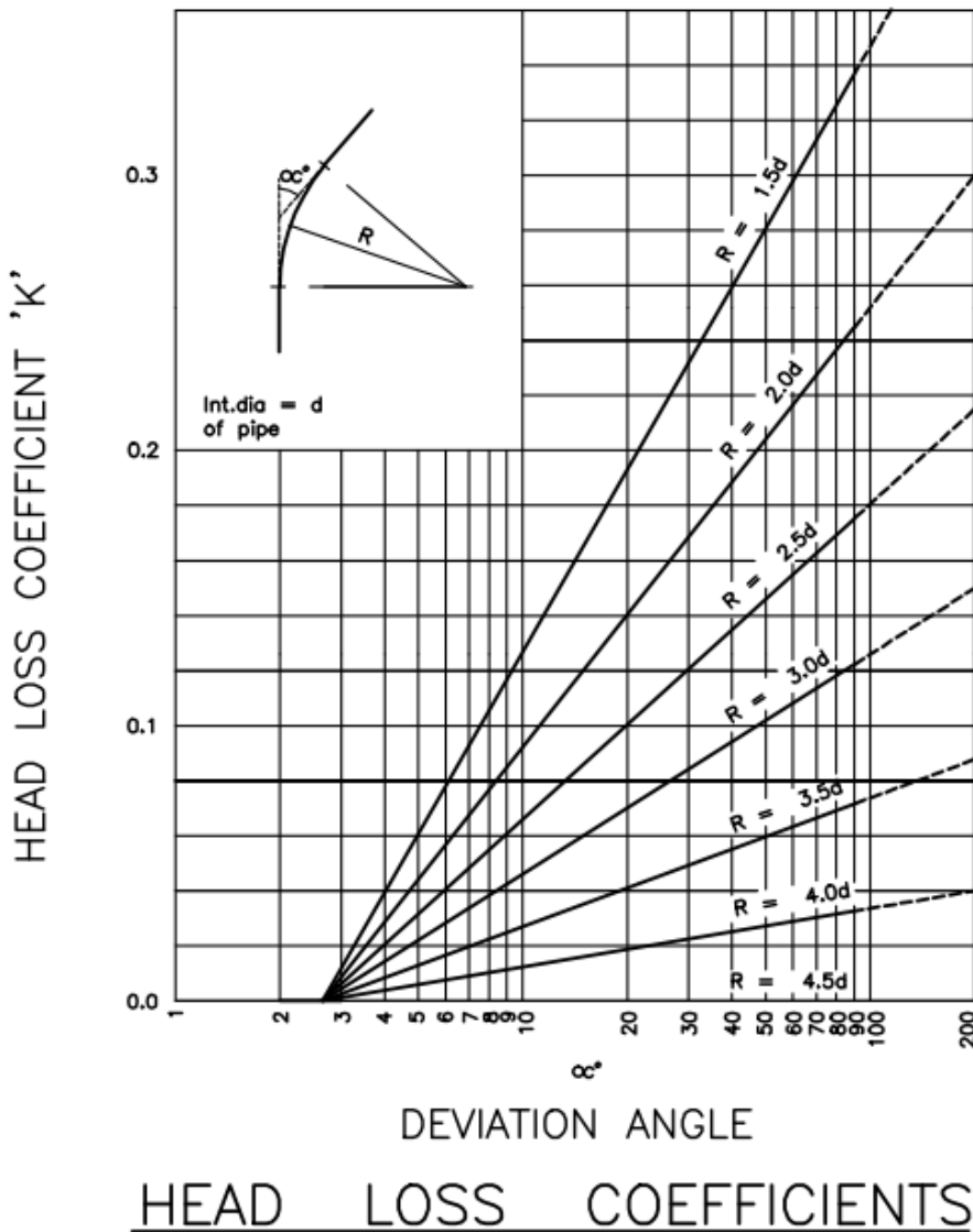
Figure 1: Head loss coefficients for bends through manholes
