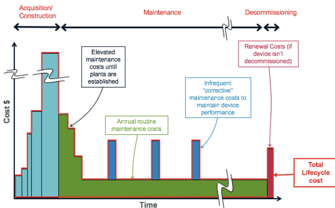
Figure 2.2 Phases in the life cycle of stormwater interventions and potential long term costs (Ira et al. , 2020)
