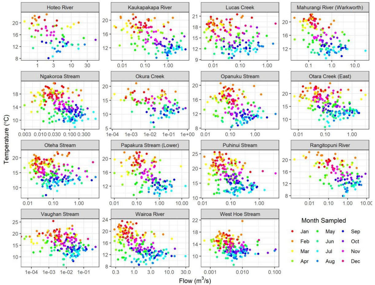
Figure 3-5: Relationships between monthly observed SOE water temperature and stream flow within individual stream sites. Data from January 2003 to June 2021. All available data used in this assessment to provide maximum number of data points at each site. Note x-axes (flow) and y-axes (temperature) are different on each plot.
