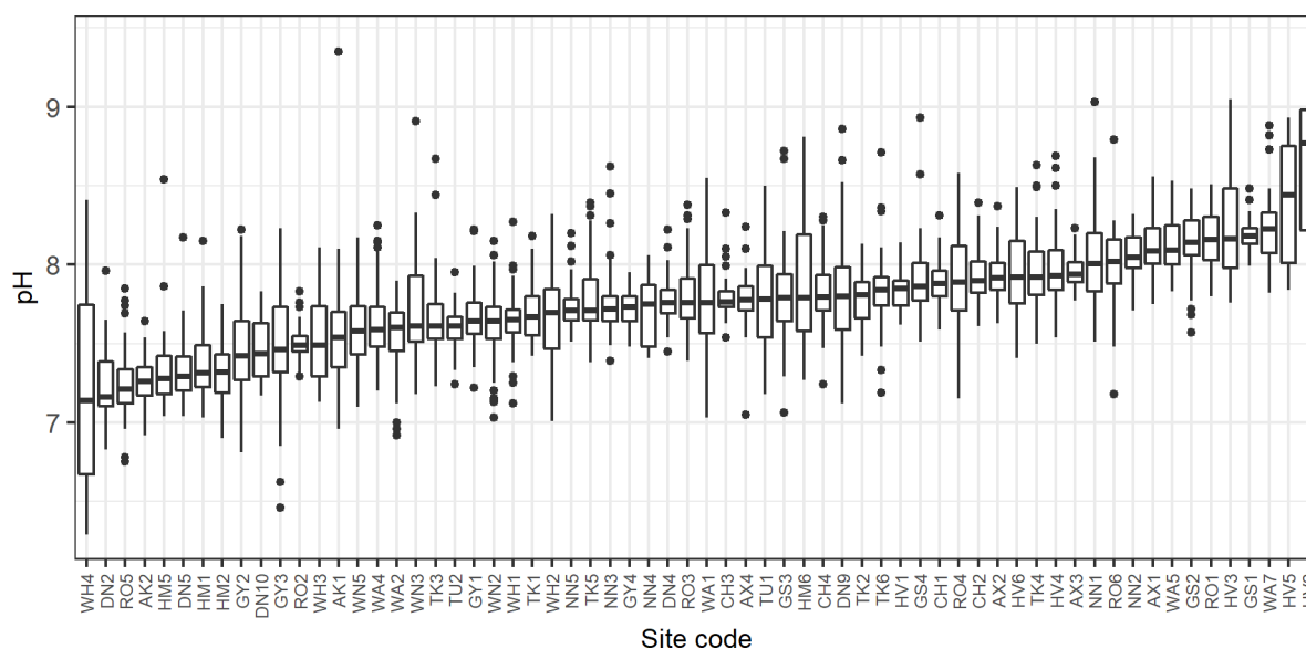
Figure 3-10: River pH from NIWA's NRWQN from 1989 to 2012.. Each box represents a specific site, sites are ordered from lowest median to highest median. pH data collected monthly, regardless of river flow. Site codes can be retrieved from https://hydrowebportal.niwa.co.nz/Data
