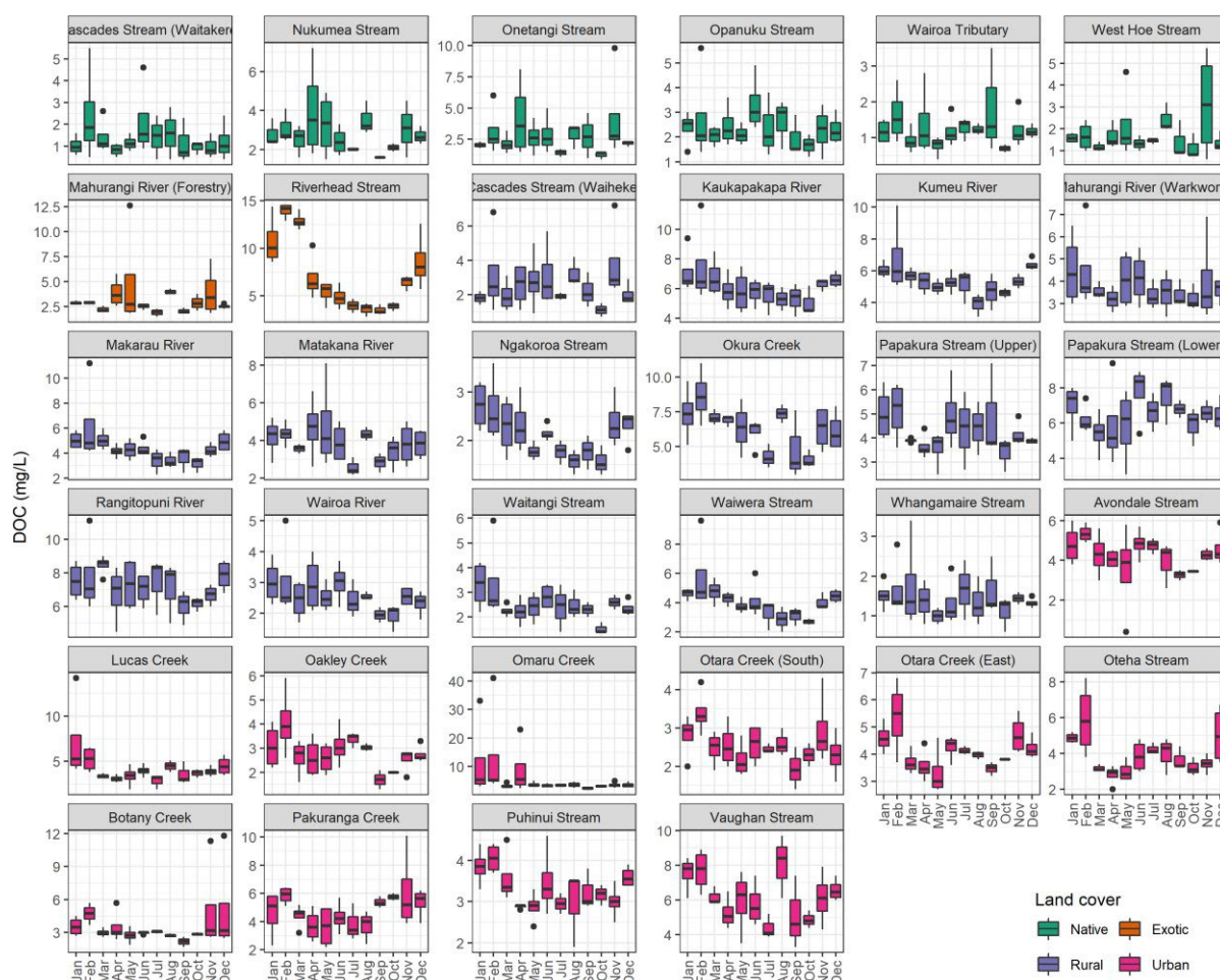
Figure 3-21: Monthly variation in DOC from SOE samples at each stream sampling site. Data from November 2017 to June 2021. All available data used in this assessment to provide maximum number of data points at each site. Note that this means the data are not evenly spread across seasons with slightly more data in summer-autumn. Note that y-axes vary on each plot. Box colour relates to the land cover in the upstream catchment.
