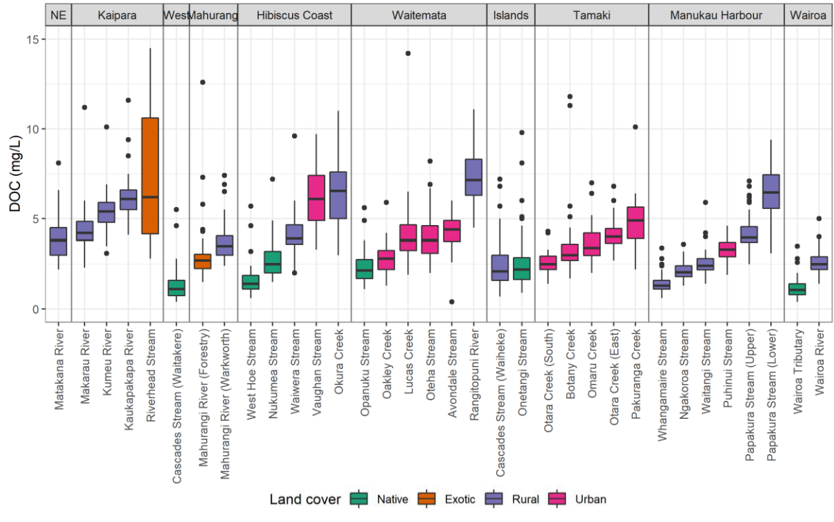
Figure 3-20: Comparison of DOC between streams based on monthly SOE Sampling. Data from November 2017 to June 2021. All available data used in this assessment to provide maximum number of data points at each site. NE = North East, West = West Coast. Within each watershed, stream sites are ordered by median DOC and coloured by land cover category. Note that three values for Omaru Stream of 23, 33 and 41 mg/L are omitted for visual clarity of other data.
