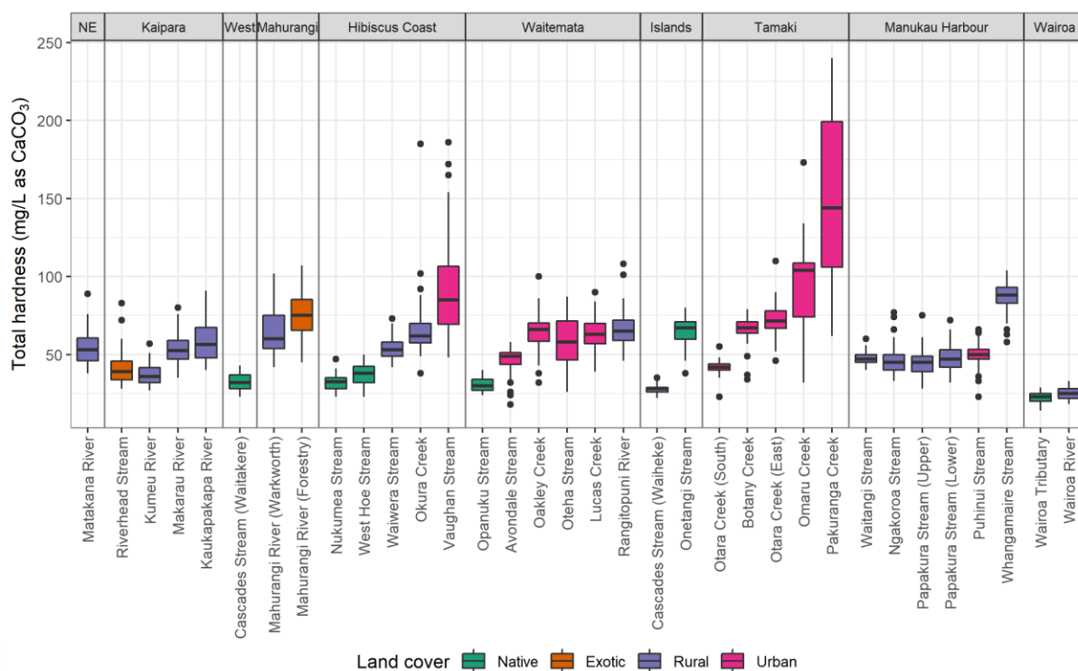
Figure 3-14: Comparison of total hardness in monthly observed SOE individual stream sites and watersheds. Data from November 2017 to June 2021. All available data used in this assessment to provide maximum number of data points at each site. NE = North East, West = West Coast. Within each watershed stream sites are ordered by median hardness and coloured by land cover category.
