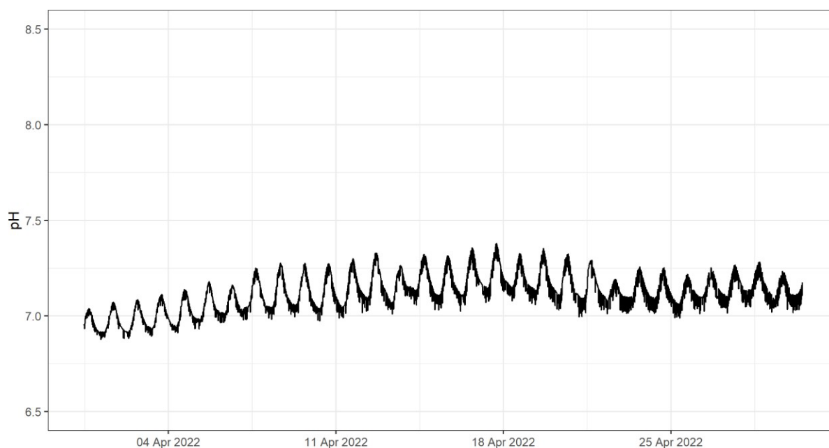
Figure 3-7: Diurnal variation in pH in Wairoa River at Tourist Road. NIWA unpublished data, as measured with YSI exo sonde, supplied by R. Davies-Colley. Larger diurnal fluctuations can be observed at sites with more primary production.
