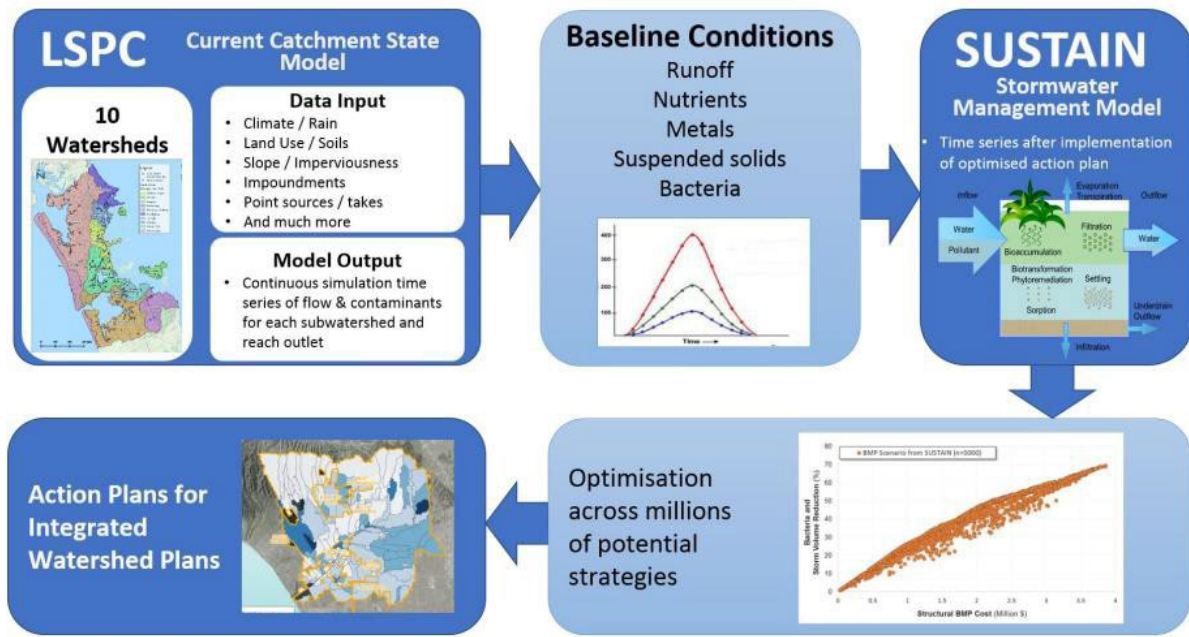
Figure 2. The FWMT is comprised of two modelling components developed by the US-EPA (LSPC and SUSTAIN) to determine current and optimized future freshwater quality state.
