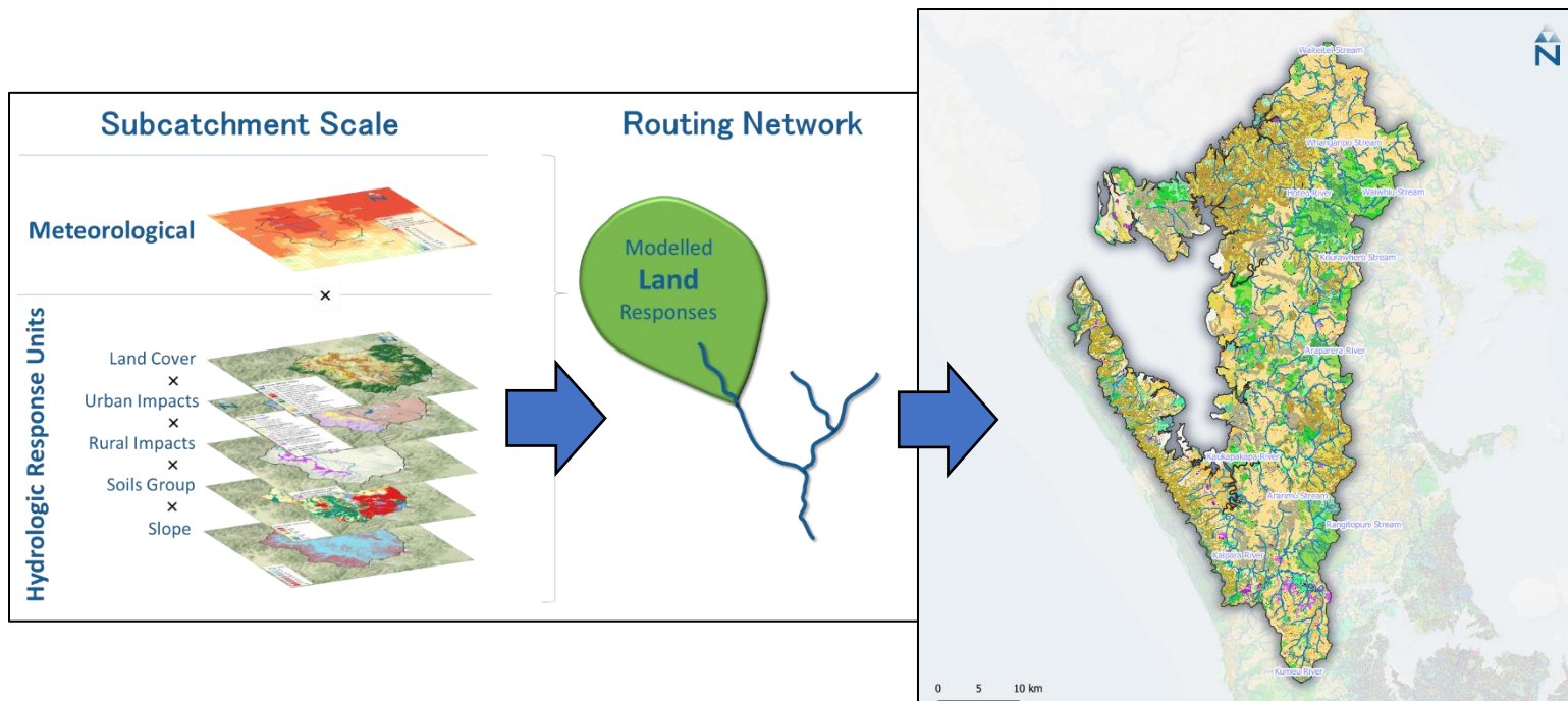
Figure 2: The FWMT’s ‘hydrologic response units’ allow for the attribution of in-stream water quality state to sub-catchment landscapes and are defined at a 2x2 m resolution across the model domain.
