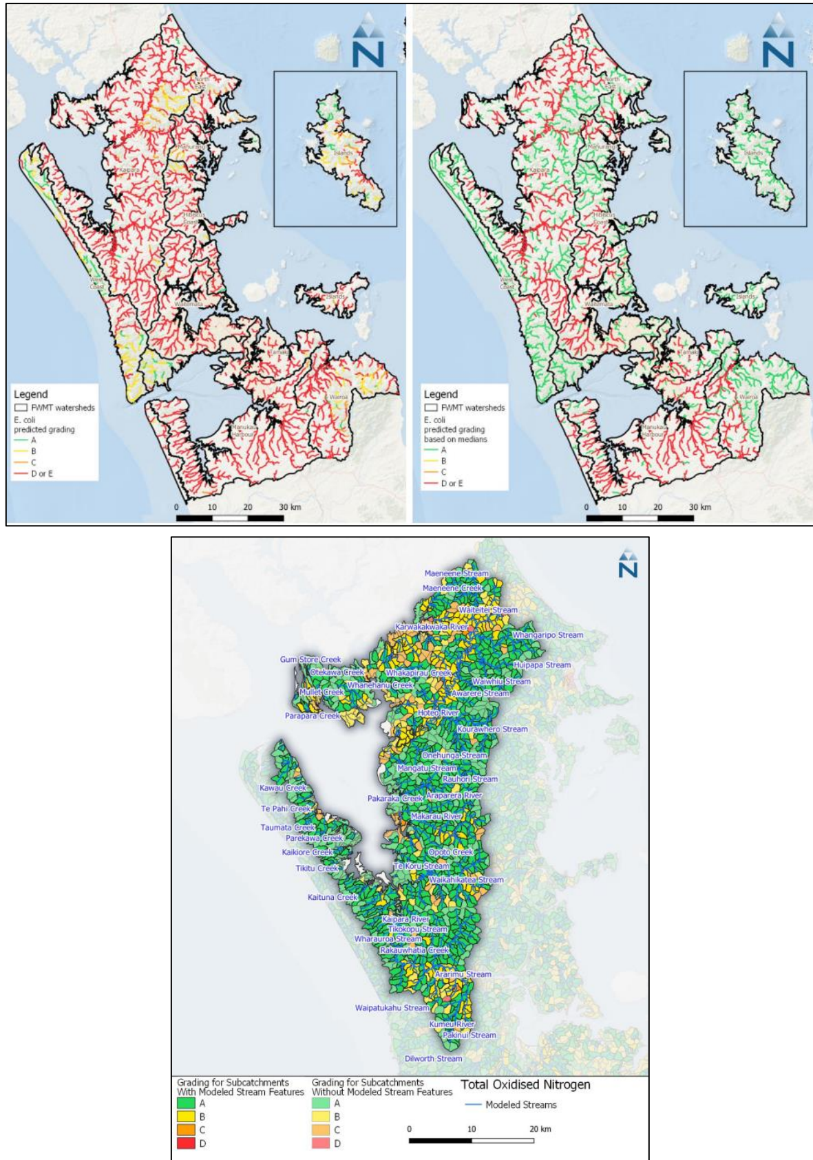
Figure 1: Top—Predicted stream grading for E.coli based on the worst performing numeric attribute state (left) and median concentration (right) (2013–2017). Bottom—Predicted sub-catchment grade for total oxidised nitrogen (TON) based on the worst performing numeric attribute state (2013–2017). Grading based on the NPS-FM (2020).
